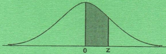
Normal Probability
